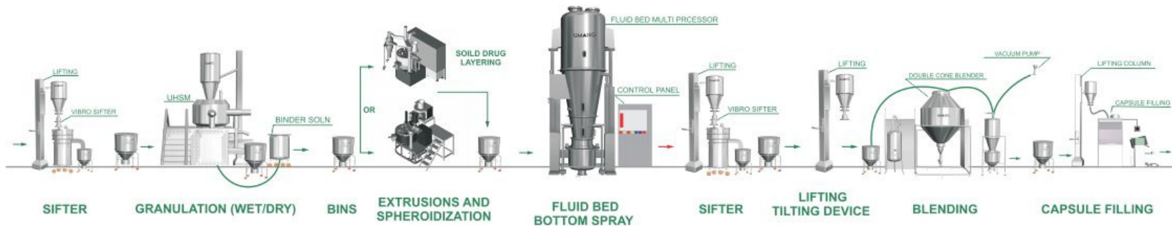
Pelletization Line
